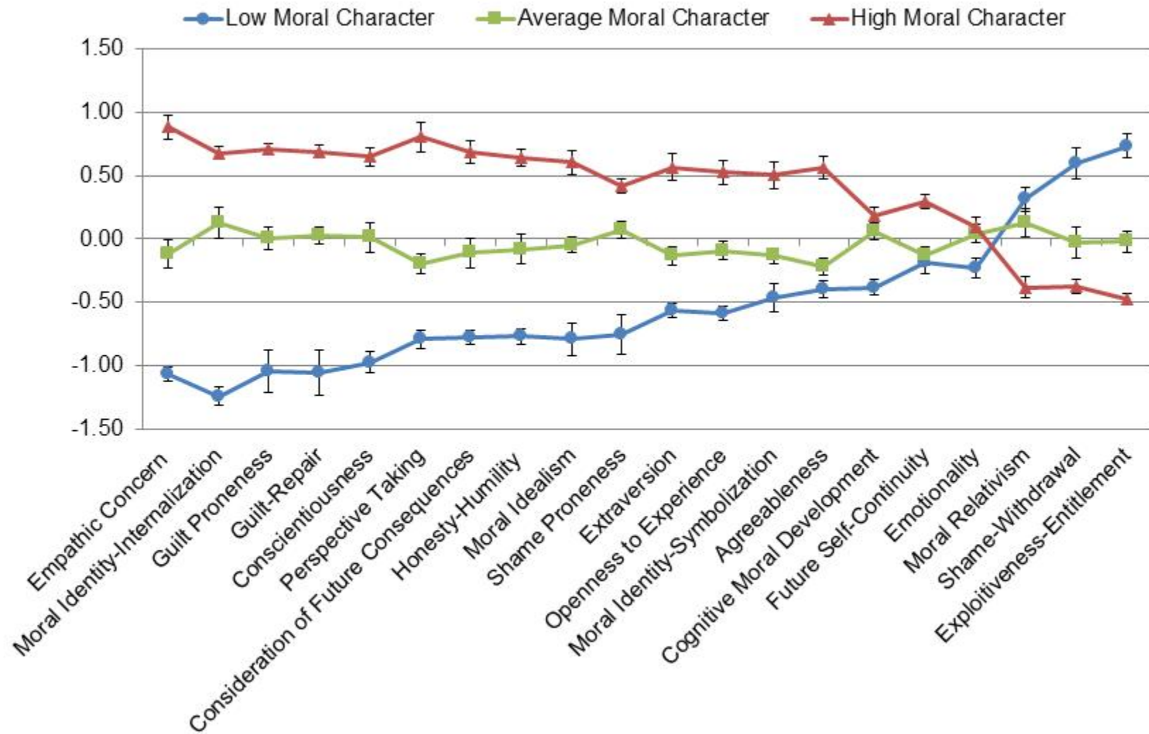
Figure 1. Study 1 ( N = 1020 ): Moral character latent profile model. Values represent the average standardized score for each variable for each latent class. Error bars denote one standard error above and below the latent class mean. 22.35% of respondents were classified as low moral character, 44.71% as average moral character, and 32.94% as high moral character.
