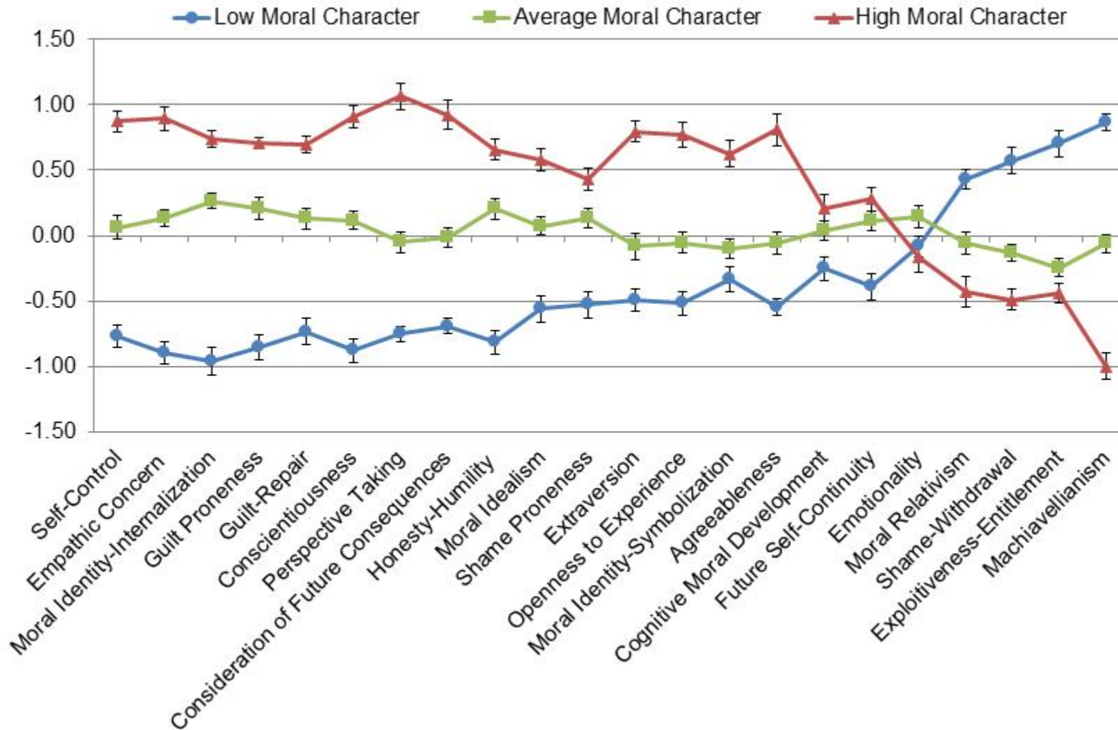
Figure 2. Study 2 ( N = 494 ): Moral character latent profile model. Values represent the average standardized score for each variable in each latent class. Error bars denote one standard error above and below the latent class mean. 30.57% of respondents were classified as low moral character, 46.36% as average moral character, and 23.08% as high moral character.
