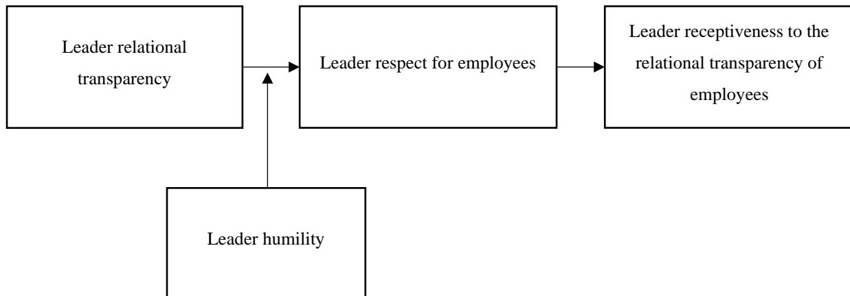
Hypothesized model
